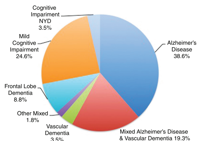
Figure 1. Cognitive diagnosis
